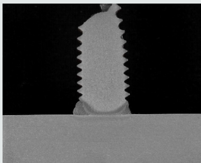
b) M10 熔融区很薄却有好的熔深 Good penetration form with a thin melting zone.
