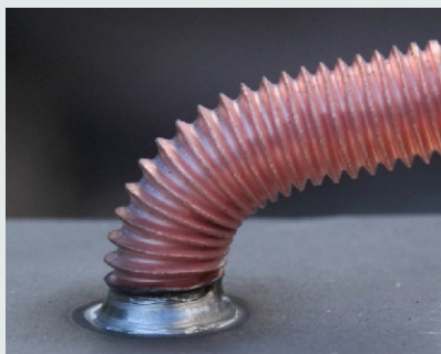
a) M8 屈曲角度: >60°测试代表成功 TEST Bending angle: >60° Test regarded as successful.
